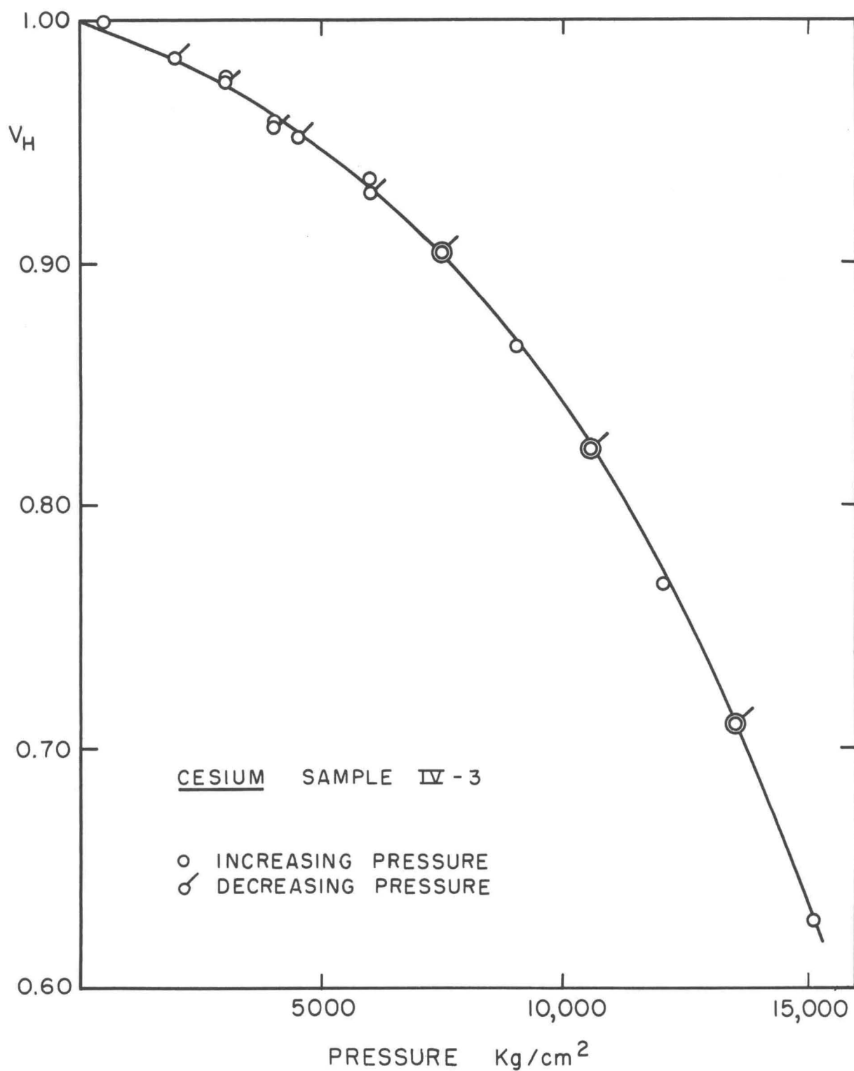
FIG. 3-9 V_H , NORMALIZED HALL VOLTAGE VS. PRESSURE
